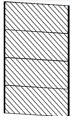
Front Maße B/H/T: 137/224/4 cm
